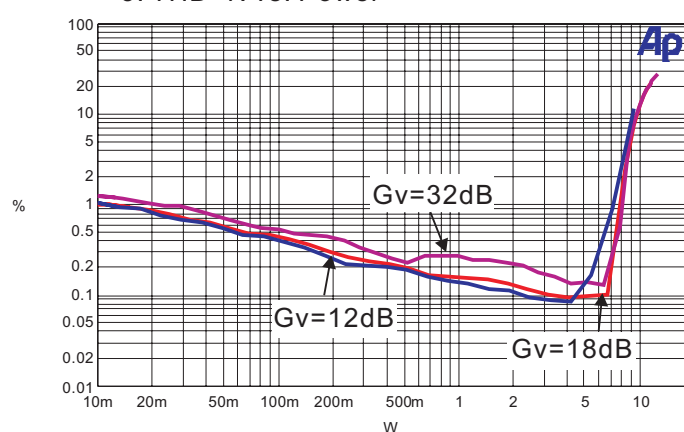
3. THD+N vs. Power
