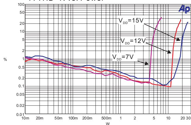
7. THD+N vs. Power
