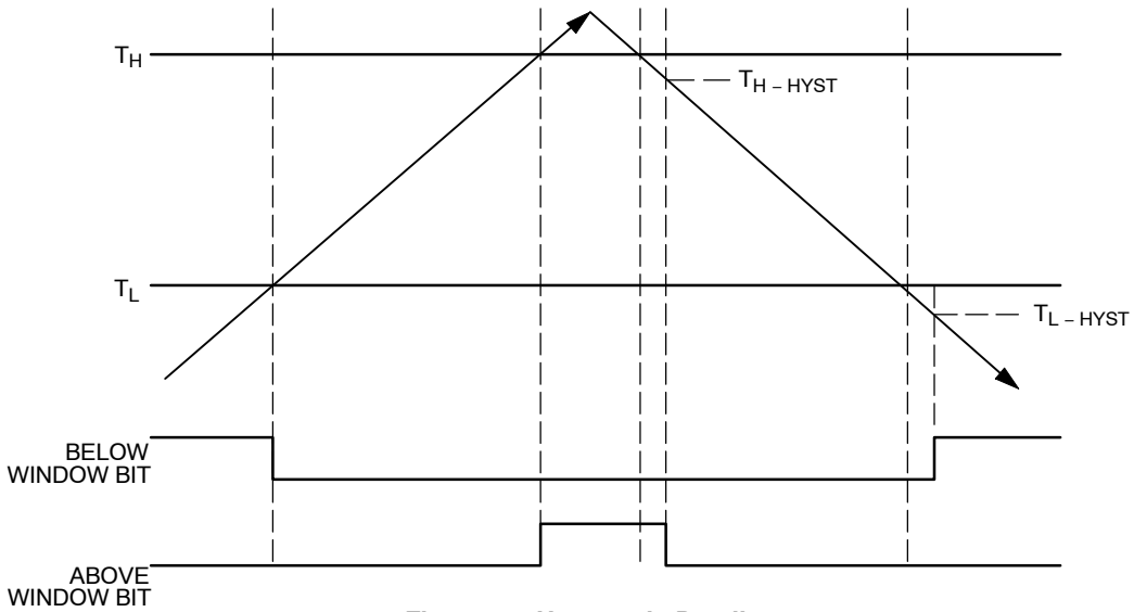
Figure 34. Hysteresis Detail
