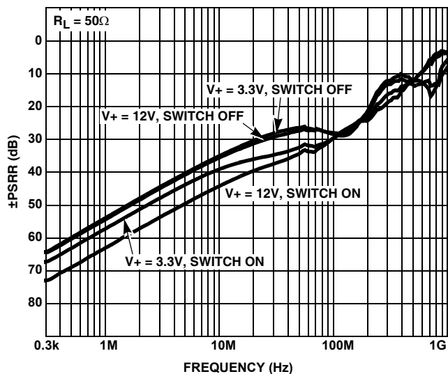
FIGURE 18. \pm\text{PSRR} vs FREQUENCY
