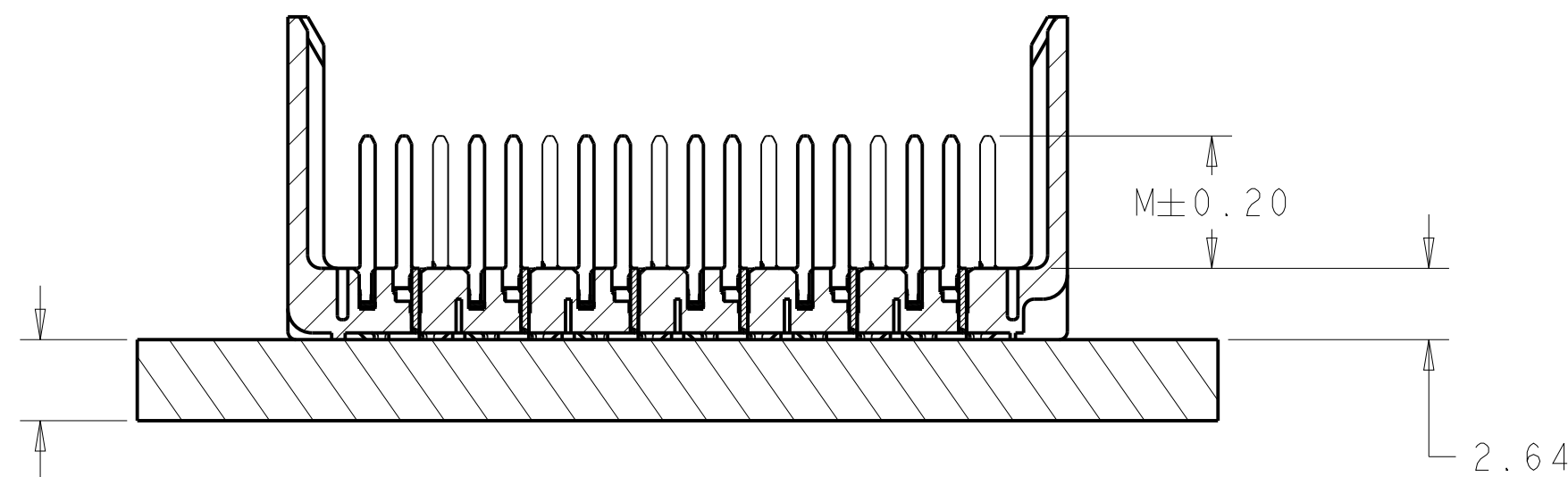
SECTION Z-Z
