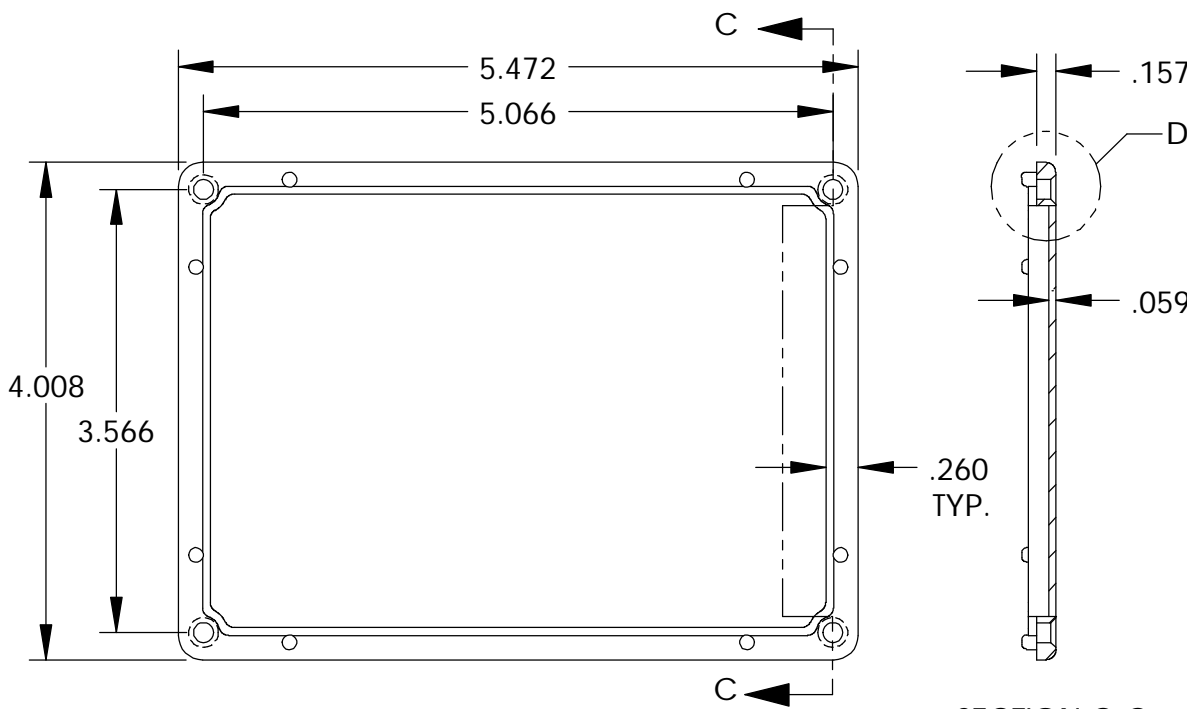
SECTION C-C
