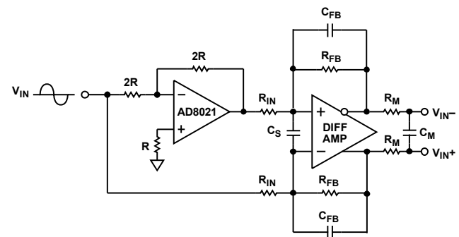
Figure 32. Single-Ended-to-Differential Conversion
