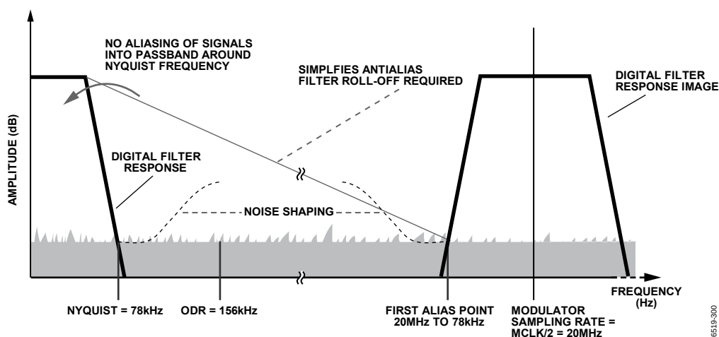
Figure 28. Antialias Example Using the AD7765 in Normal Mode, Decimate 128× Using MCLK/2 = ICLK = 20\text{ MHz}
