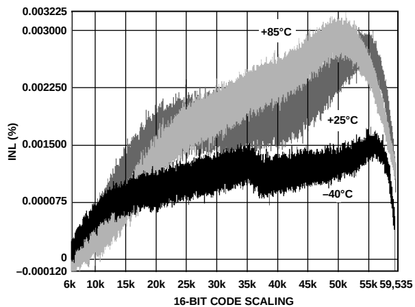
Figure 21. Low Power Mode INL
