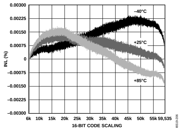
Figure 18. Normal Power Mode INL
