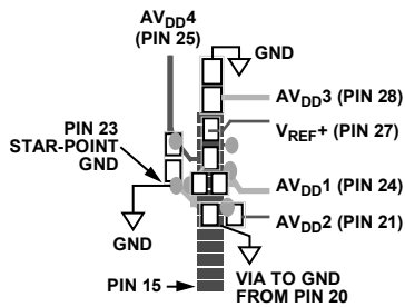
Figure 46. AD7765 Supply Decoupling
