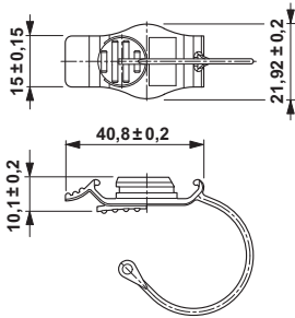
Dimensioned drawing
