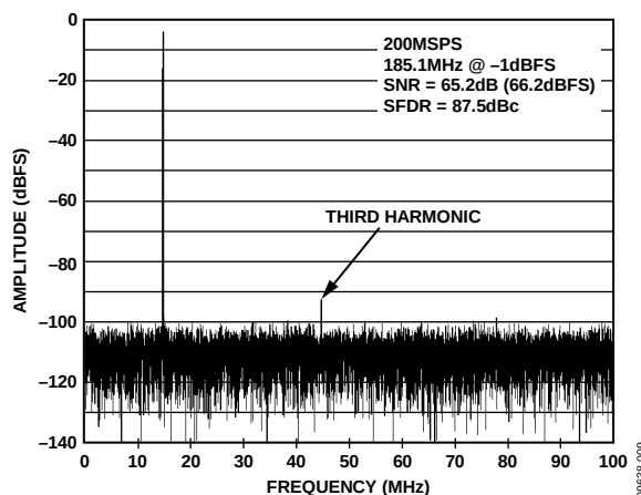
Figure 9. AD6643-200 Single Tone FFT, f_{IN} = 185.1 MHz
