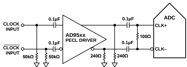
Figure 49. Differential PECL Sample Clock (Up to 625 MHz)
