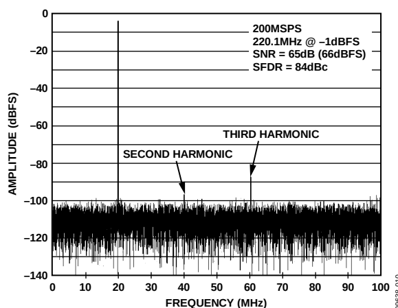
Figure 10. AD6643-200 Single Tone FFT, f_{IN} = 220.1 MHz
