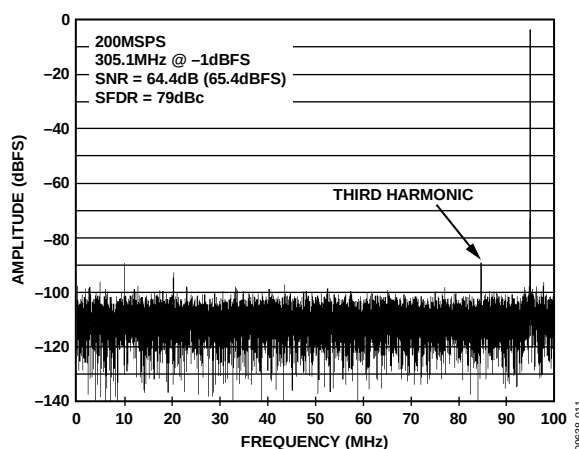
Figure 11. AD6643-200 Single Tone FFT, f_{IN} = 305.1 MHz
