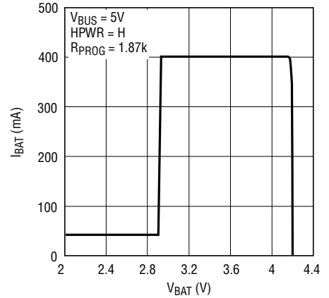
I_{\text{BAT}} vs V_{\text{BAT}} (LTC3554/LTC3554-2/LTC3554-3)
