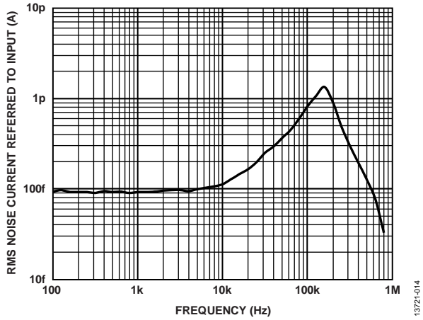
Figure 10. Noise Bandwidth/Peaking
