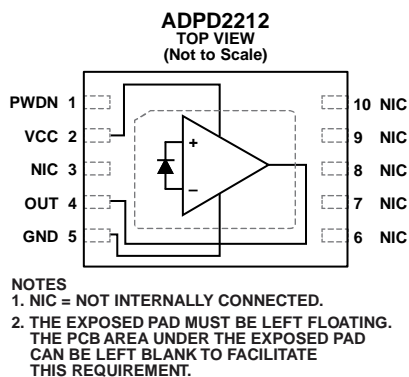
Figure 3. Pin Configuration
