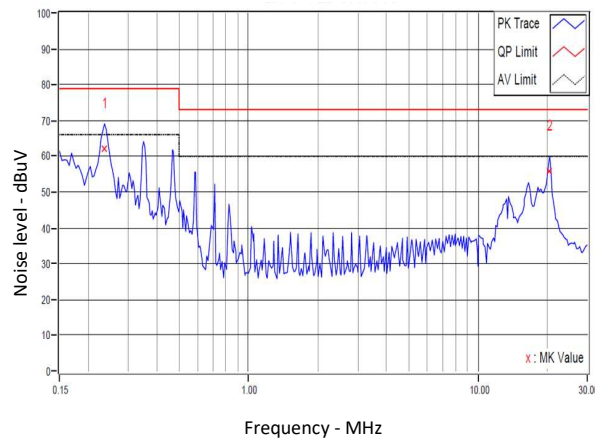
Figure 12. Conducted Emissions
