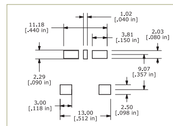
P.C. MOUNTING
