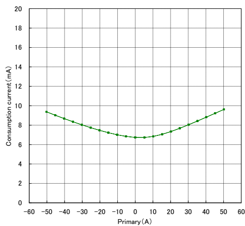
Fig.9-3 Consumption Current
