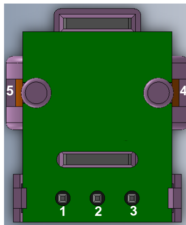
Fig.6-2 Pin assignment
