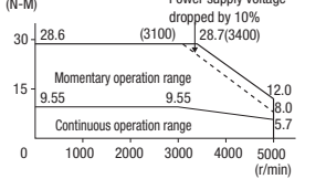
R88M-K3K030F/C (3 kW)
