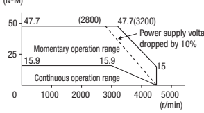
R88M-K5K030F/C (5 kW)
