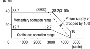
R88M-K4K030F/C (4 kW)
