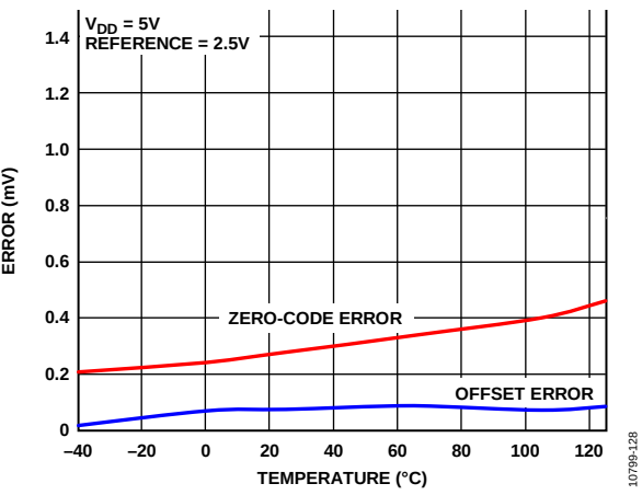
Figure 13. Zero-Code Error and Offset Error vs. Temperature
