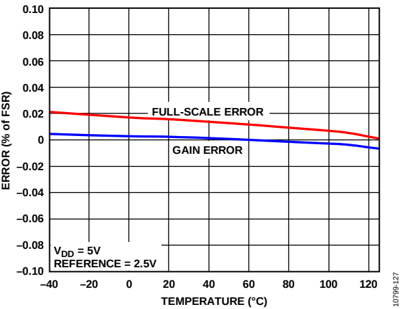
Figure 12. Gain Error and Full-Scale Error vs. Temperature
