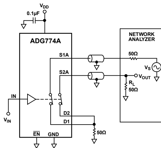
Figure 21. Channel-to-Channel Crosstalk
