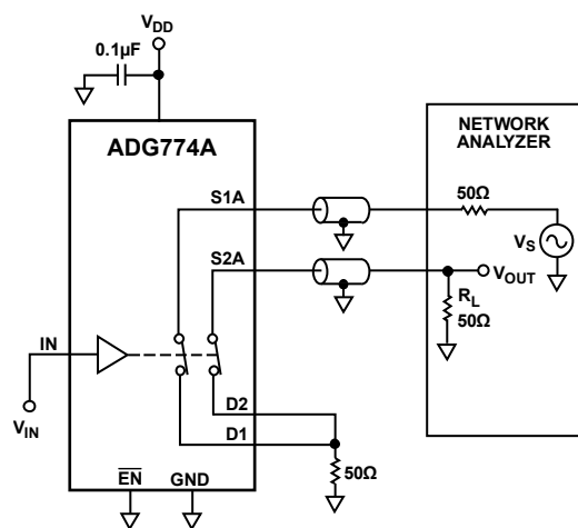
Figure 21. Channel-to-Channel Crosstalk
