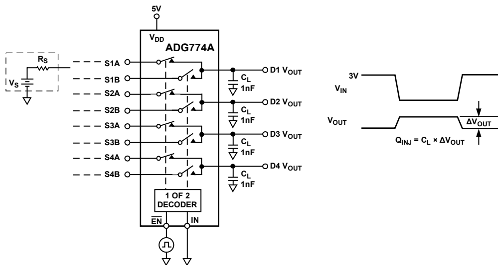
Figure 24. Charge Injection
