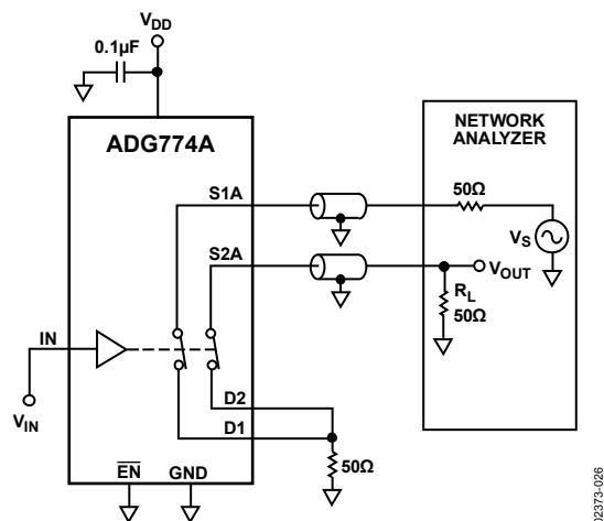
Figure 21. Channel-to-Channel Crosstalk
