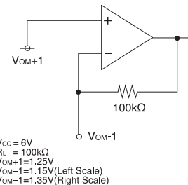
Fig. 27 Test Circuit
