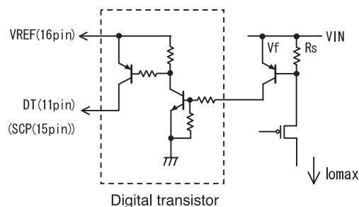
Typical covercurrent protection circuit Fig.40
