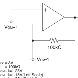
Fig. 30 Test Circuit
