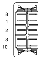
BOTTOM VIEW TERMINAL ARRANGEMENT 10 TERMINAL BASE
