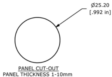
Panel Cutout SPDT & DPDT
