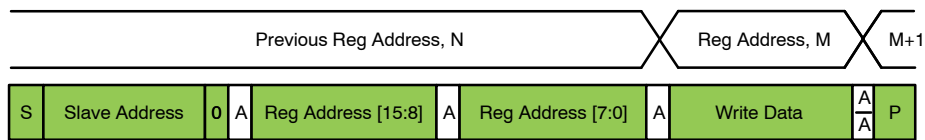
Figure 33. Single WRITE to Random Location
