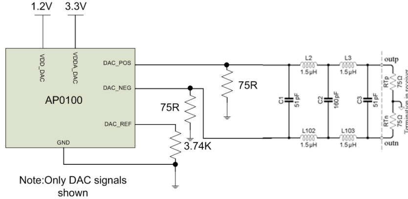
Figure 27. Differential Connection
