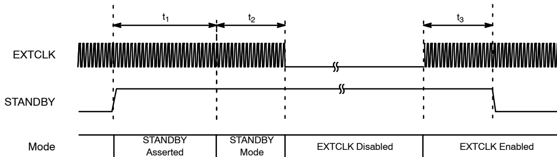
Figure 8. Hard Standby Operation
