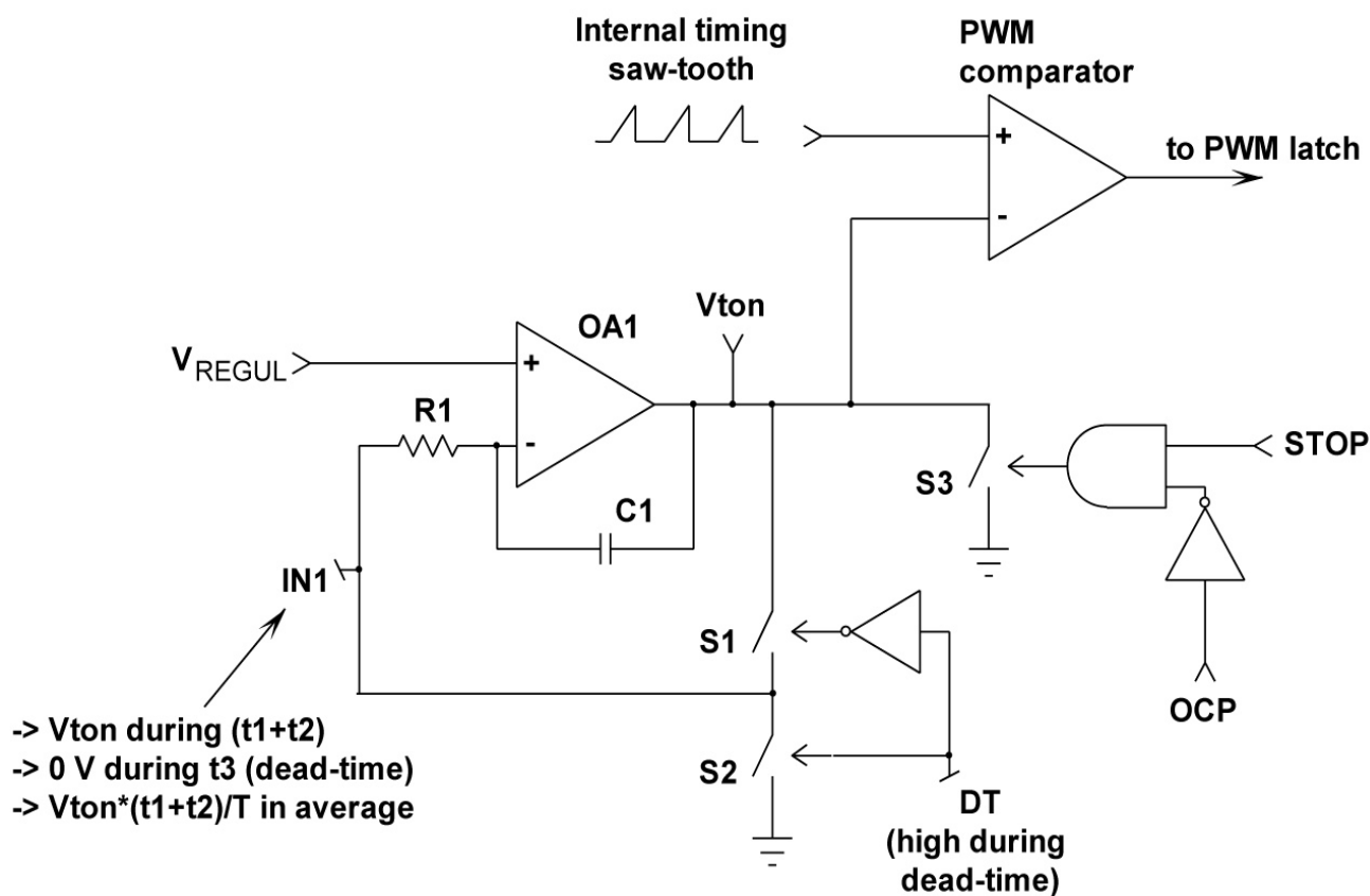
Figure 66. V_{TON} Processing Circuit. The integrator OA1 amplifies the error between V_{REGUL} and IN1 so that on average, (V_{TON} \cdot (t_1+t_2)/T) equates V_{REGUL} .
