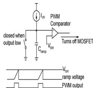
Figure 65. PWM circuit and timing diagram.
