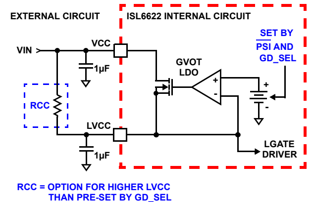
FIGURE 2. GATE VOLTAGE OPTIMIZATION (GVOT) DETAIL
