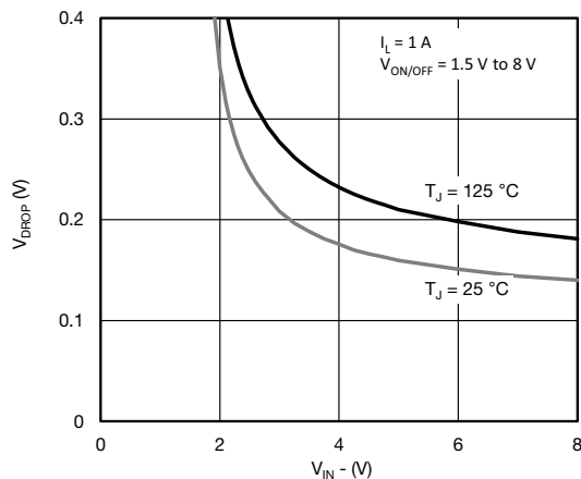
V_{DROP} vs. V_{IN} at I_L = 1\text{ A}
