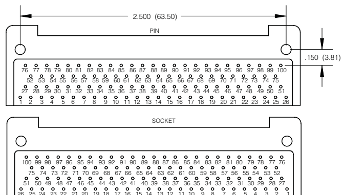
100 CONTACTS
