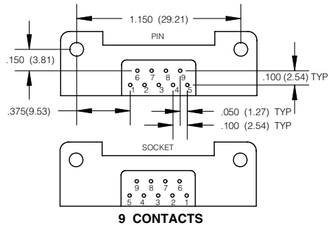
9 CONTACTS
