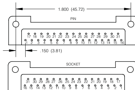
31 CONTACTS
