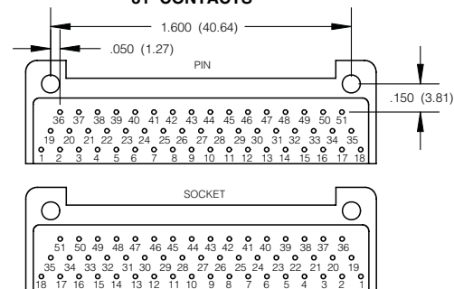
51 CONTACTS
