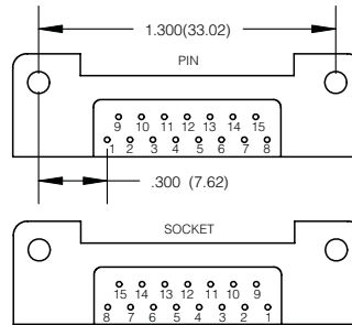
15 CONTACTS
