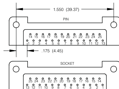
25 CONTACTS
