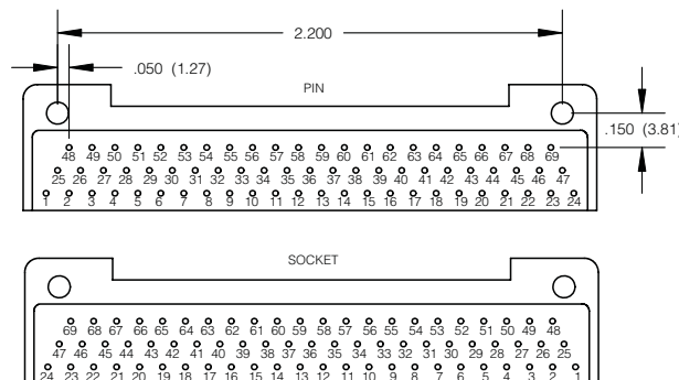
69 CONTACTS
