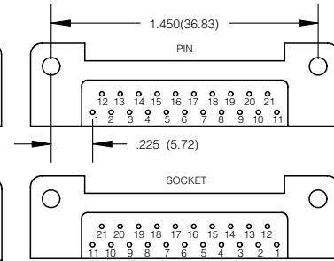
21 CONTACTS
