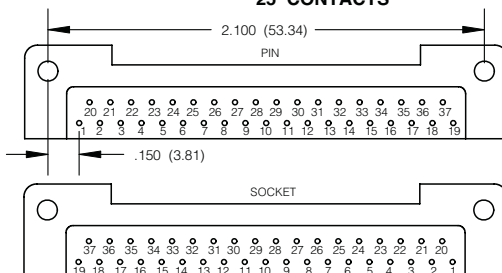
37 CONTACTS
