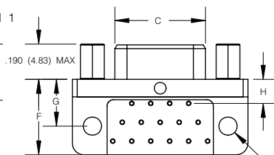
VIEW SHOWN FOR 9, 15, 21, AND 25 CONTACT ARRANGEMENTS
