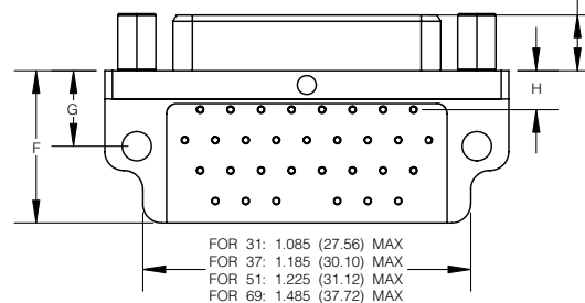
VIEW SHOWN FOR 31, 37, 51 and 69 CONTACT ARRANGEMENTS
