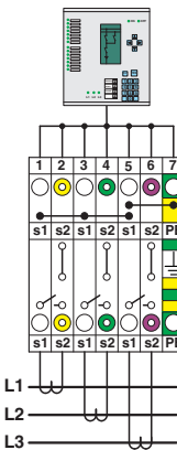
Interlinked three-phase current transformer set with grounded star point
