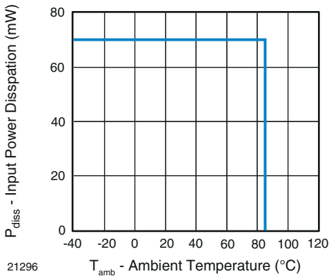
Fig. 1 - Input Power Dissipation vs. Ambient Temperature
