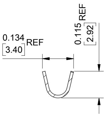
SECTION A-A INSULATION CRIMP
