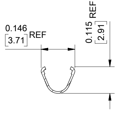
SECTION B-B CONDUCTOR CRIMP
