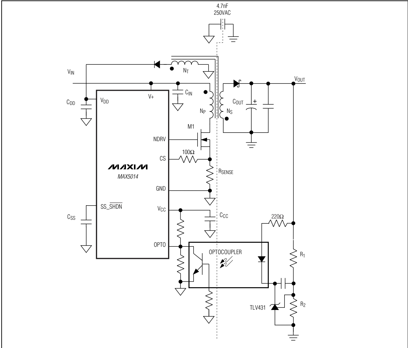
Figure 3. Flyback Converter
