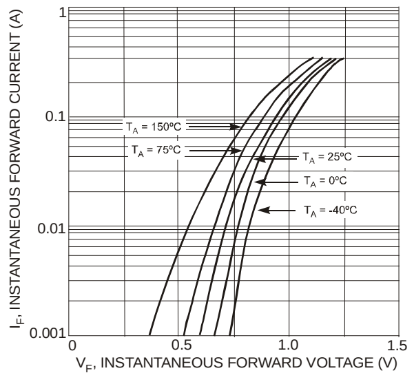
Fig. 2 Forward Characteristics
