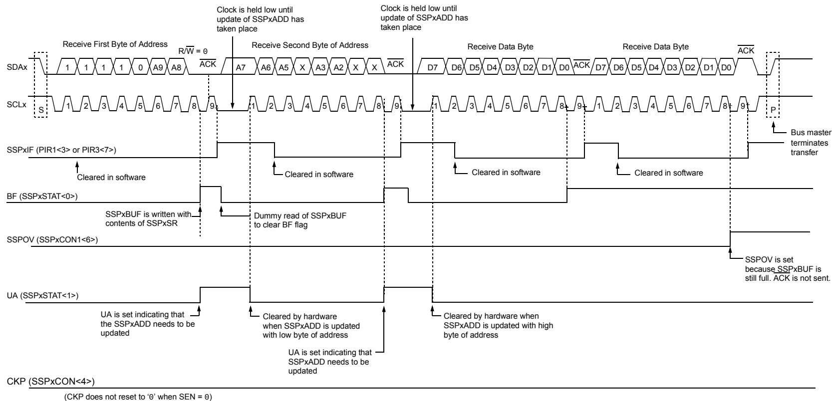
FIGURE 20-11: I 2 C SLAVE MODE TIMING WITH SEN = 0 AND MSK<5:1> = 01001 (RECEPTION, 10-BIT ADDRESS)
