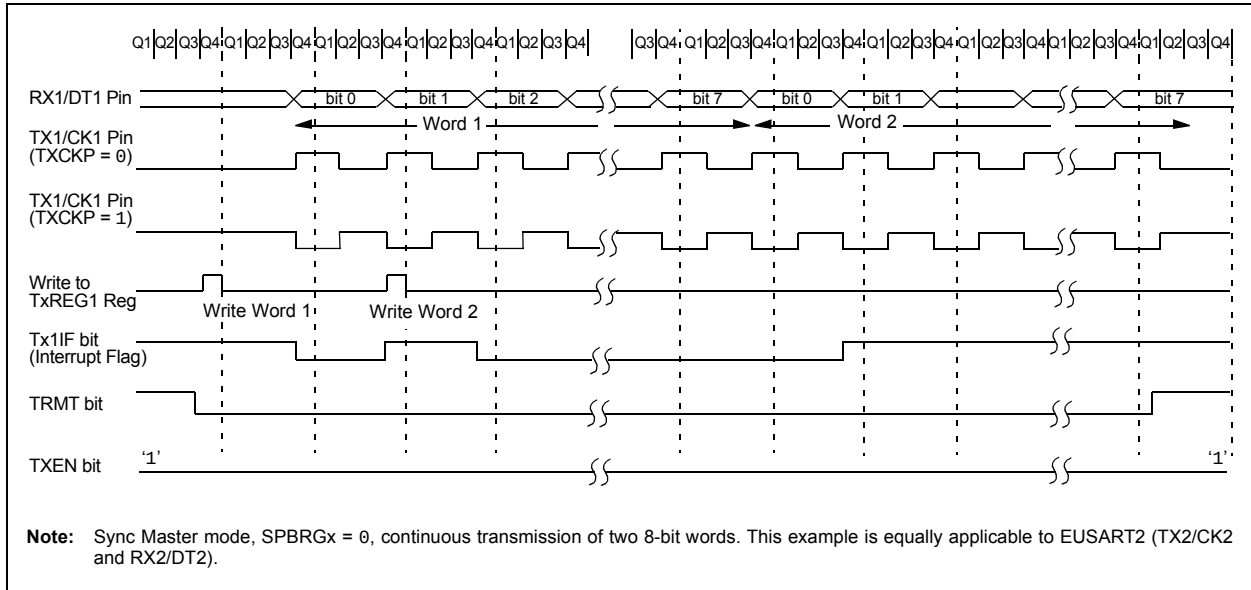
FIGURE 21-11: SYNCHRONOUS TRANSMISSION
