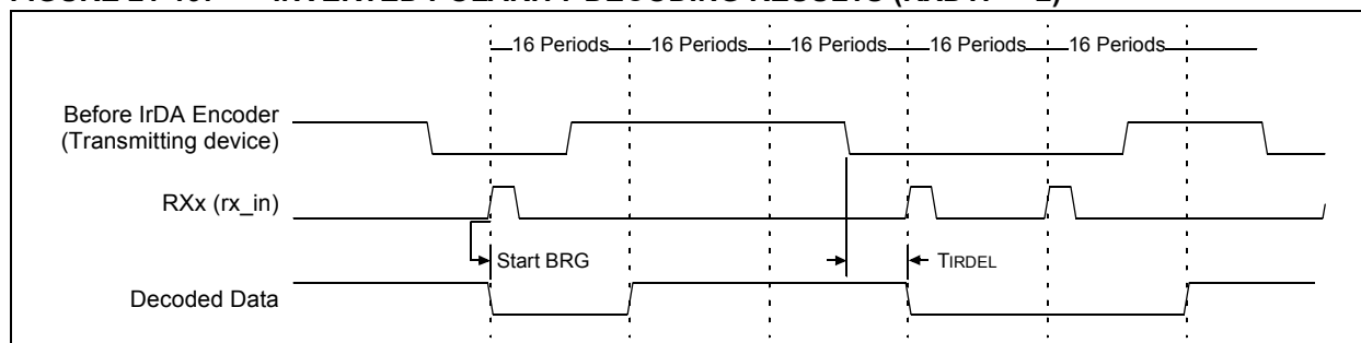
FIGURE 21-19: INVERTED POLARITY DECODING RESULTS (RXDTP = 1)
