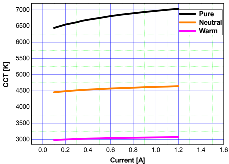
CCT vs. Forward Current, T_a = 25^\circ\text{C}
