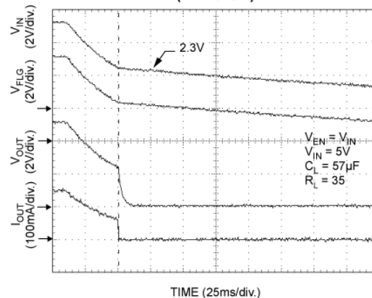
UVLO— V_{IN} Falling (MIC2025-1)
