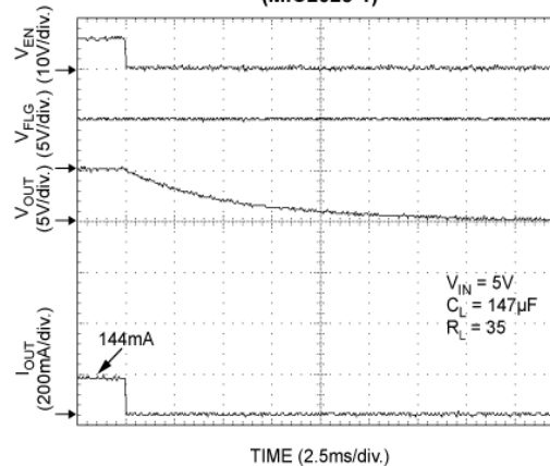
Turn-off Response (MIC2025-1)
