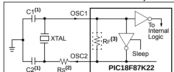
FIGURE 3-4: CRYSTAL/CERAMIC RESONATOR OPERATION (HS OR HSPLL CONFIGURATION)
