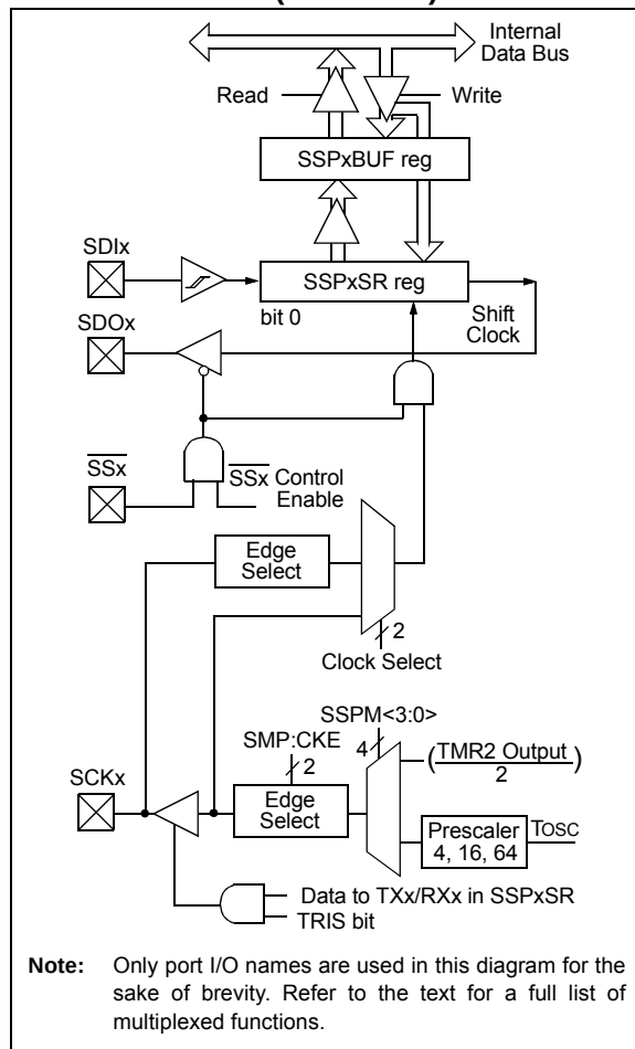
FIGURE 21-1: MSSP BLOCK DIAGRAM (SPI MODE)
