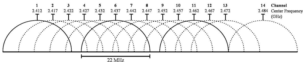
Figure 3 WLAN channels
