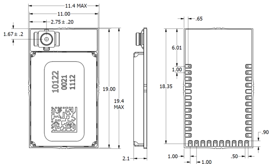
Figure 11 A2530E24C dimensions
