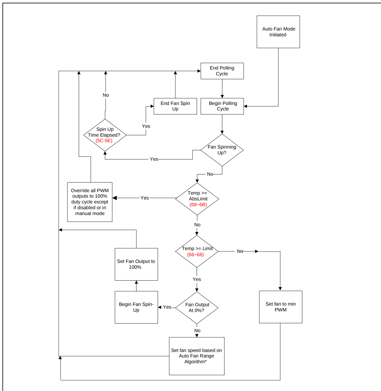
FIGURE 21-4: AUTOMATIC FAN CONTROL FLOW DIAGRAM
