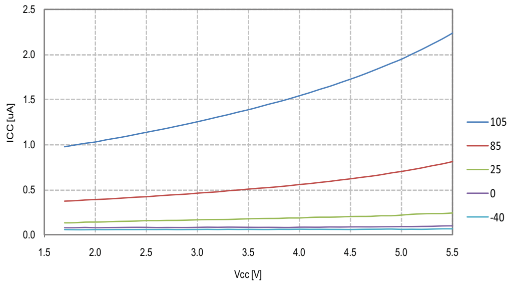
Figure 26-19.Power-down Supply Current vs. V_{CC} , Watchdog Timer Disabled
