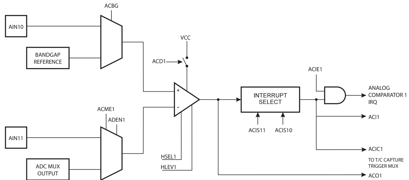
Figure 15-1. Analog Comparator 1 Block Diagram
