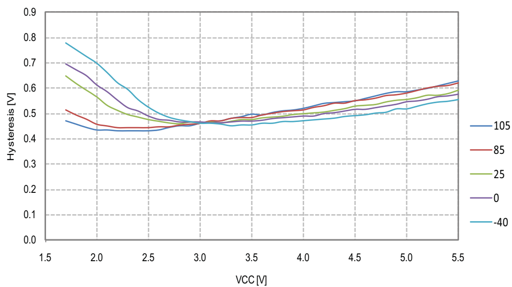
Figure 26-137.Reset Pin as I/O Input Hysteresis vs. V_{CC}
