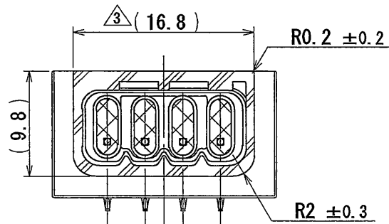
SECT. Y-Y
