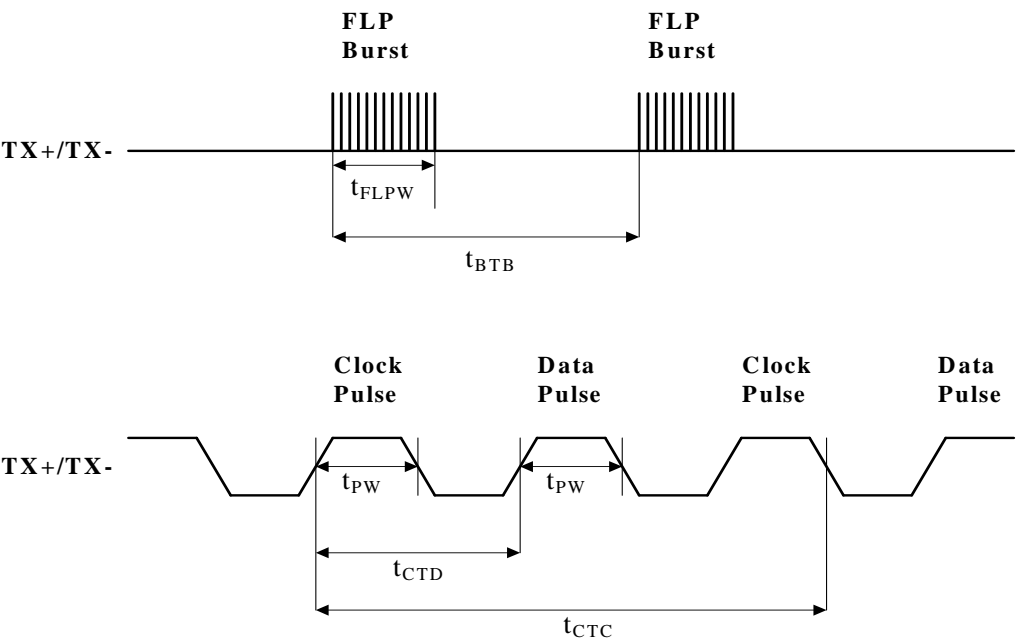
Figure 27. Auto-Negotiation Timing
