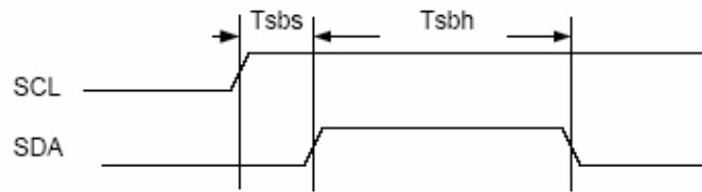
Figure 23. I2C Stop Bit Timing
