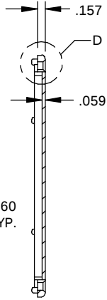
SECTION C-C
