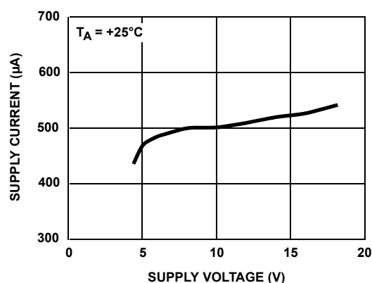
FIGURE 10. EL5420 SUPPLY CURRENT PER AMPLIFIER vs SUPPLY VOLTAGE
