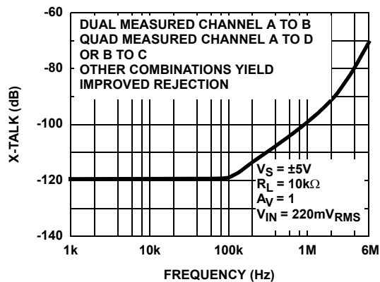
FIGURE 20. CHANNEL SEPARATION vs FREQUENCY RESPONSE
