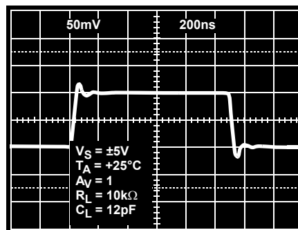
FIGURE 24. SMALL SIGNAL TRANSIENT RESPONSE
