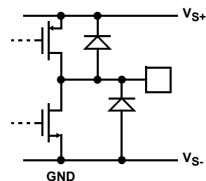
CIRCUIT 2
