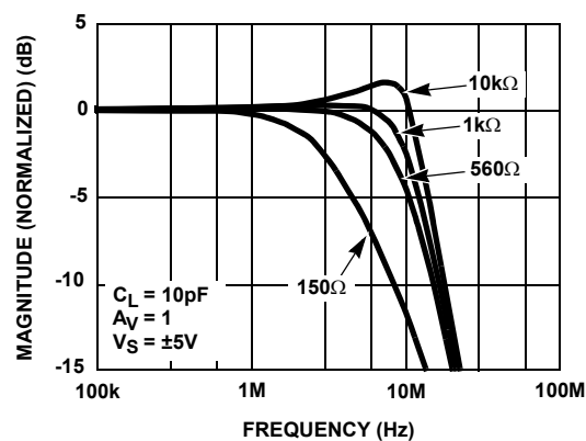
FIGURE 12. FREQUENCY RESPONSE FOR VARIOUS R_L
