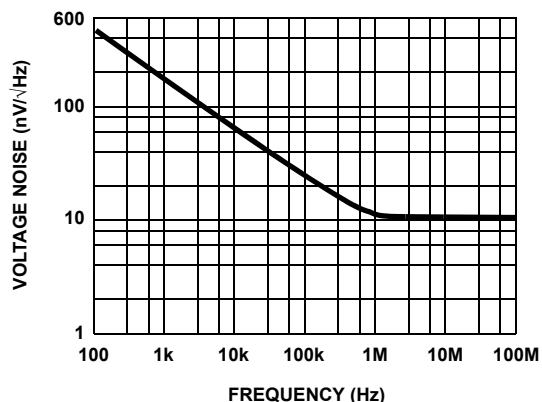
FIGURE 18. INPUT VOLTAGE NOISE SPECTRAL DENSITY vs FREQUENCY
