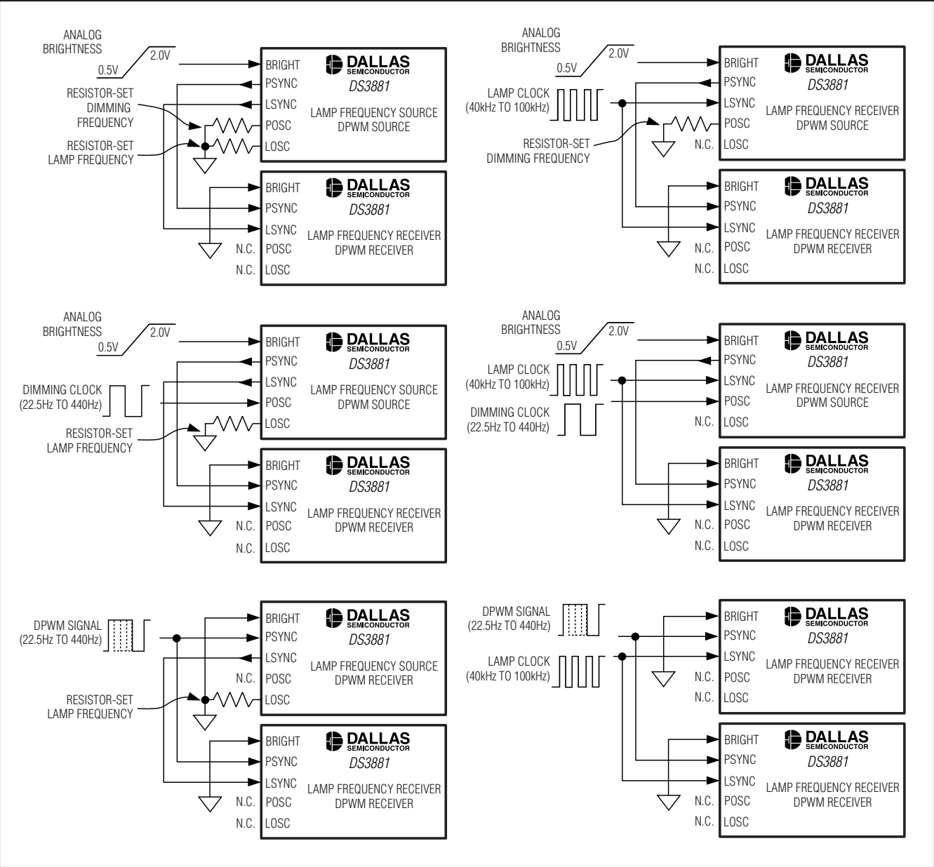
Figure 5. Frequency Configuration Options for Designs Using Multiple DS3881s
