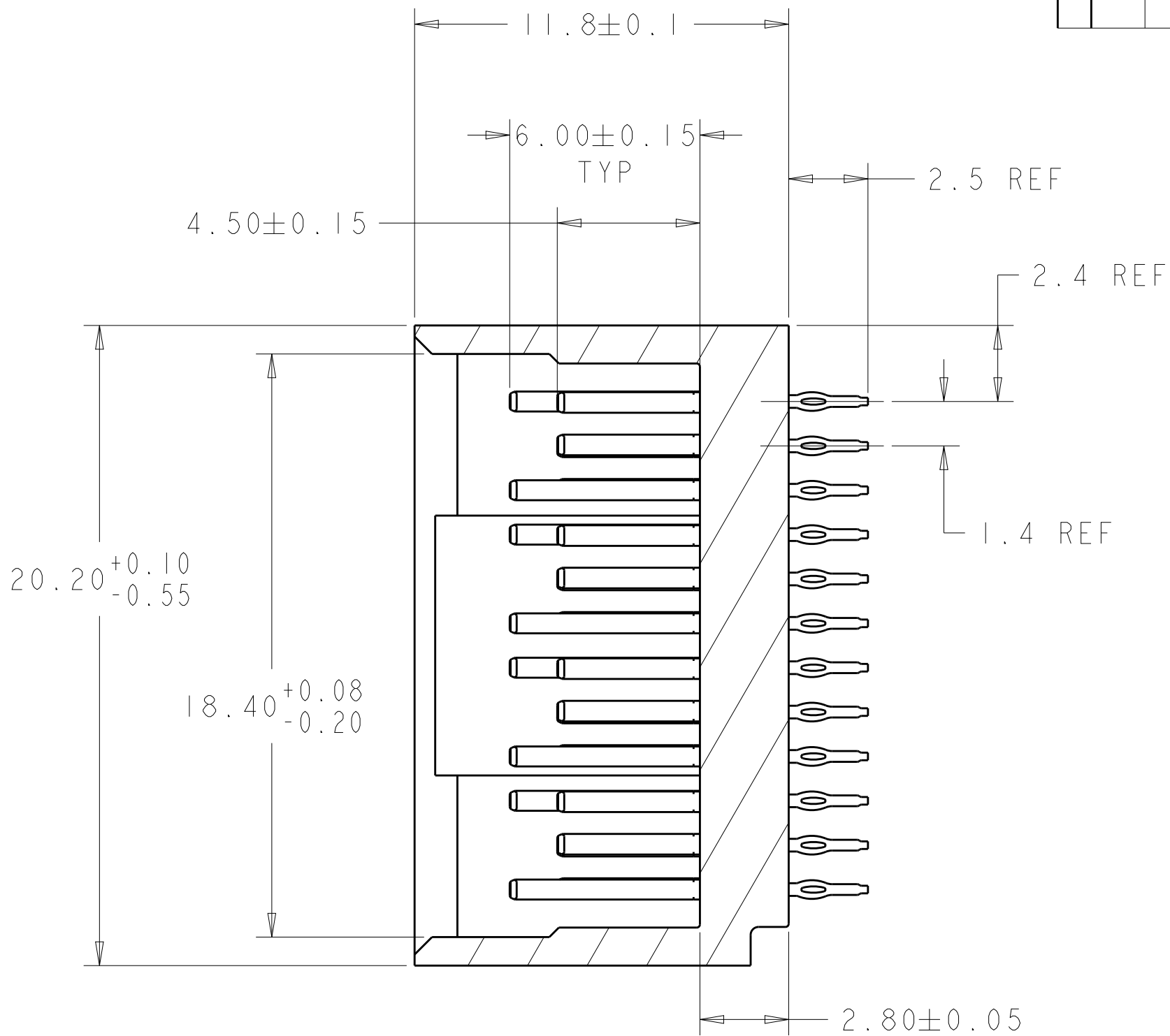
SECTION W-W
