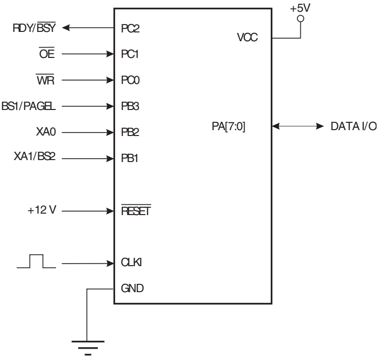
Figure 23-1. Parallel Programming Signals
