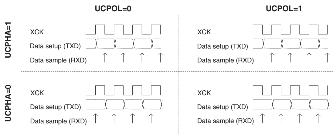
Figure 17-1. UCPHAN and UCPOLn data transfer timing diagrams.
